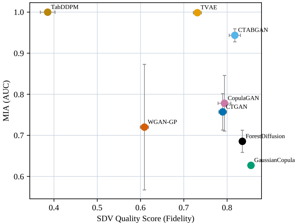
Bank Marketing: SDV Quality Score (Fidelity) vs MIA (AUC)
